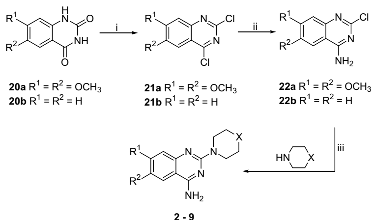
Scheme 1. Experimental conditions: (i) POCl_3 , PCl_5 , PhN(CH_3)_2 , reflux, 20 h; (ii) 35% NH_4OH , THF, rt, 16 h; (iii) appropriate amine, 1-pentanol or isoamyl alcohol, reflux, 3–20 h.
