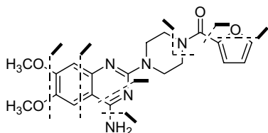
Figure 3. Notional fragmentations of the prazosin structure.
