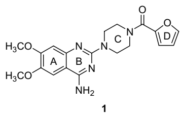
Figure 2. The four rings, labelled A–D, in prazosin ( 1 ).
