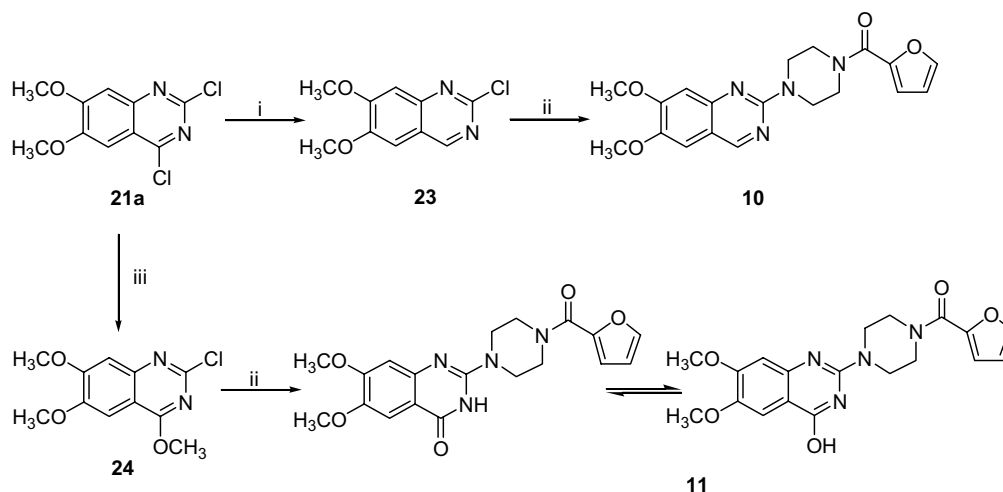
Scheme 2. Experimental conditions: (i) NaBH 4 , isopropanol, 70–80 °C, 5 days; (ii) 1-(2-furoyl)piperazine, isoamyl alcohol, 150 °C, 18 h; (iii) NaOCH 3 , CH 3 OH, reflux, 12 h.
