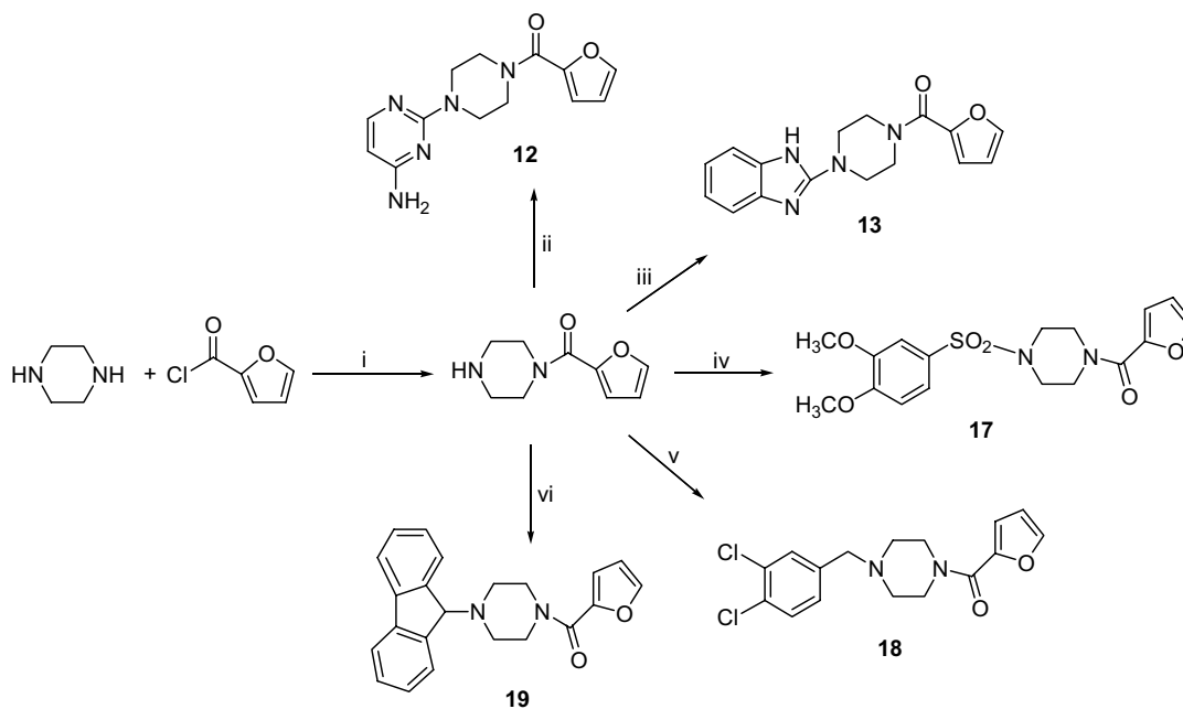
Scheme 3. Experimental conditions: (i) 48% HBr, EtOH–H 2 O, 80 °C, 1.5 h; (ii) 4-amino-2-chloropyrimidine, 1-pentanol, reflux, 3 h; (iii) 2-chlorobenzimidazole, 1-pentanol, 100 °C, 6 h; (iv) 3,4-dimethoxybenzene sulfonyl chloride, Et 3 N, CH 2 Cl 2 , rt, 12 h; (v) 3,4-dichlorobenzyl bromide, 1-pentanol, reflux, 16 h; (vi) 9-bromofluorene, 1-pentanol, reflux, 12 h.
