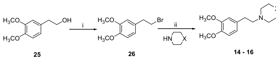
Scheme 4. Experimental conditions: (i) PPh 3 , N -bromosuccinimide, toluene, rt, 12 h; (ii) appropriate amine, K 2 CO 3 , EtOH, reflux, 24 °C.
